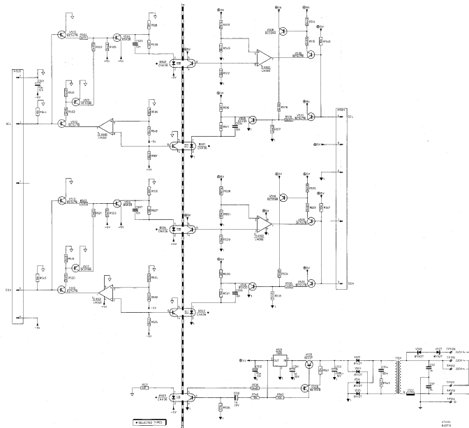
Fig. 7.15. Galvanic separation
