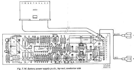
Fig. 7.14. Battery power supply p.c.b., lay-out, conductor side
