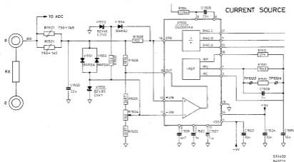
Fig. 2.6. Ohm measurements
